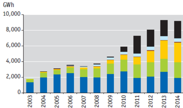
Chart 1 → Electricity generation from RES in the Czech Republic [GWh], 2003–2014
